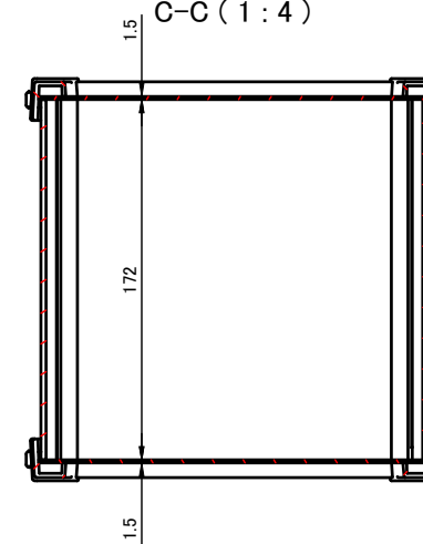
C-C (1:4)
